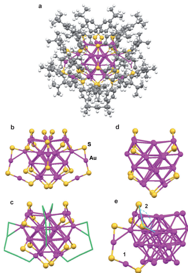
Figure 2. Total structure of [\text{Au}_{36}(\text{SPh-}t\text{Bu})_{24}]^0 . a) The entire particle (Ph- t Bu = gray atoms), b) the \text{Au}_{36}\text{S}_{24} framework, c) the four dimeric staples shown in green, d) the \text{Au}_{28}\text{S}_{12} framework, e) comparison of the ostensible dimeric staple (labeled 2 ) and the standard dimeric staple (labeled 1 ).
